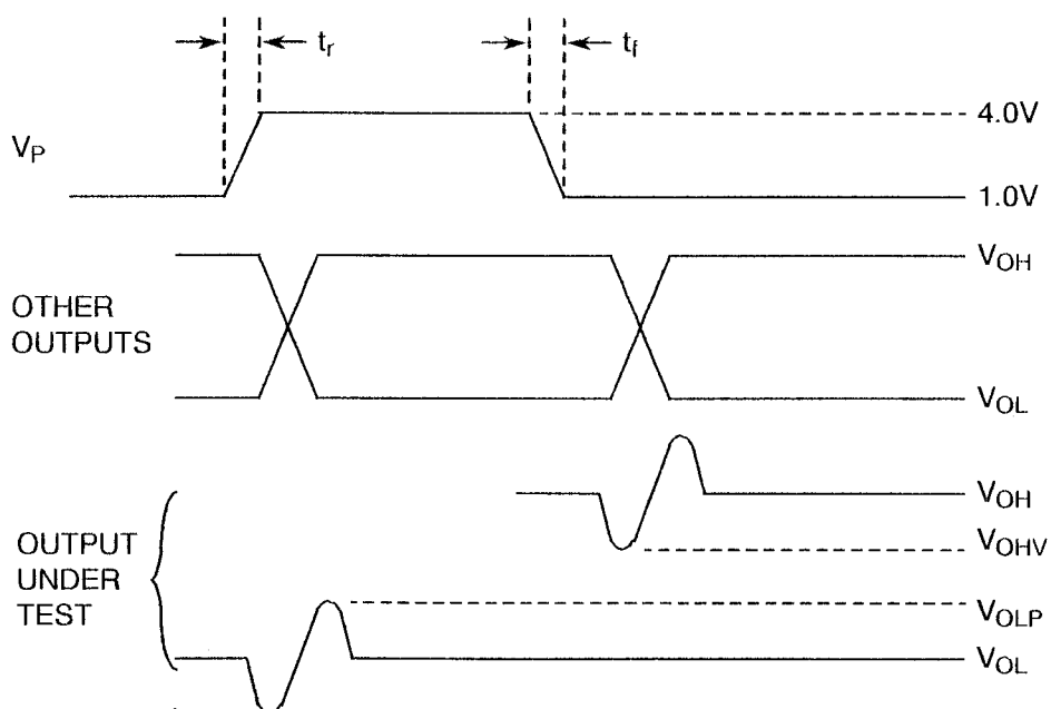
VOLTAGE WAVEFORMS
