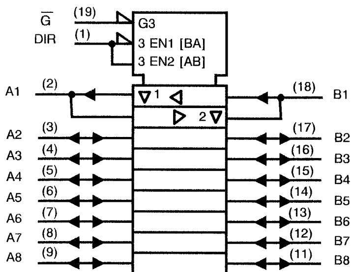
FIGURE 3(d) - FUNCTIONAL DIAGRAM
