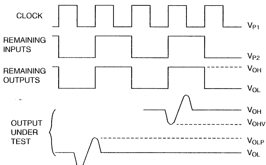
VOLTAGE WAVEFORMS
