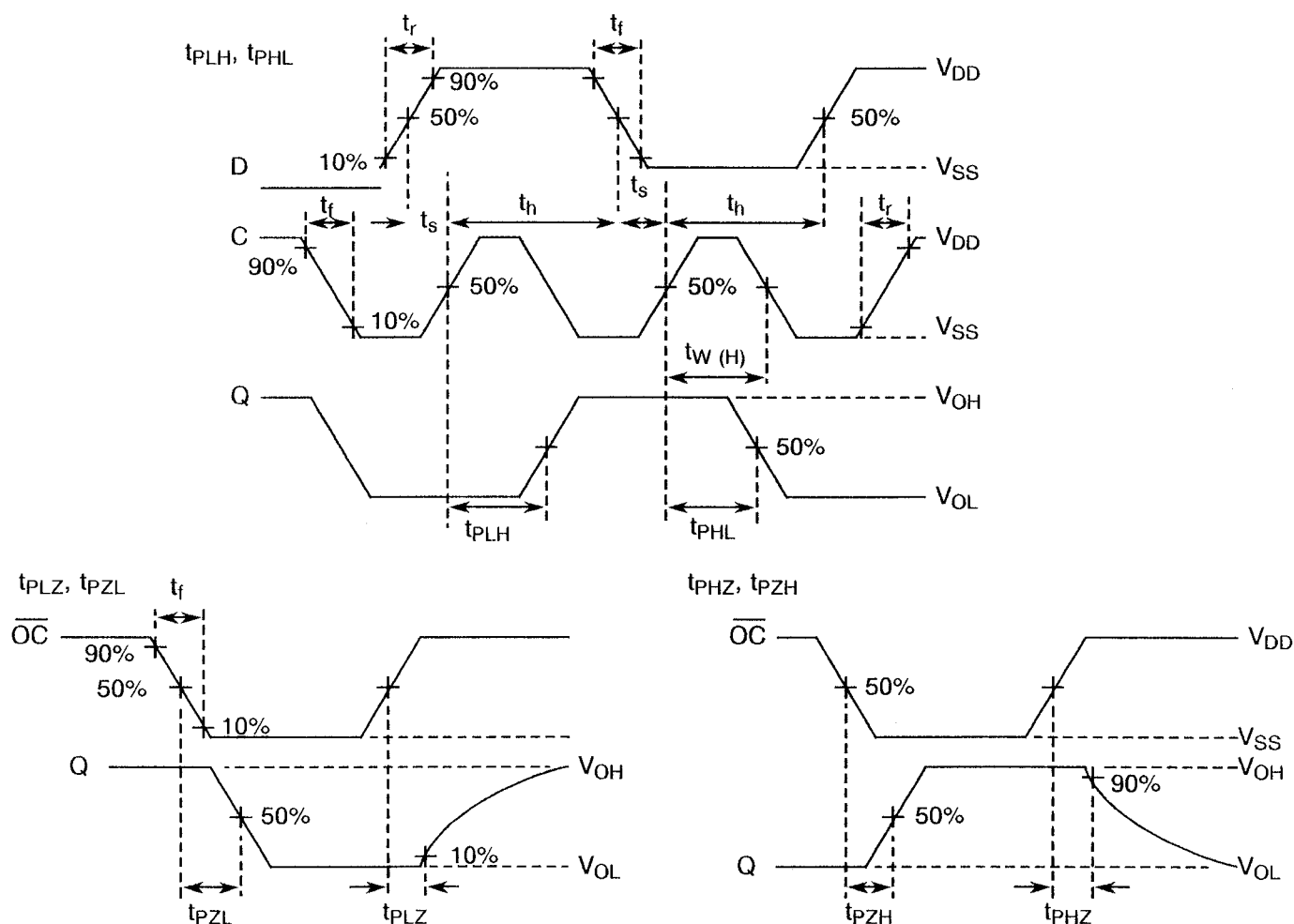
VOLTAGE WAVEFORMS
