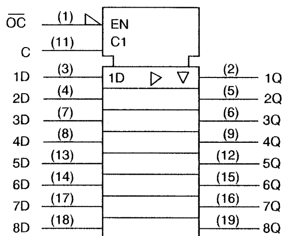
FIGURE 3(d) - FUNCTIONAL DIAGRAM
