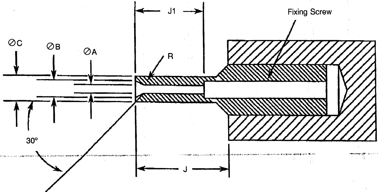
FIGURE 3 - GAUGE FIXTURE
