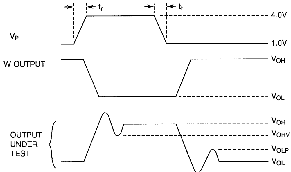
VOLTAGE WAVEFORMS
