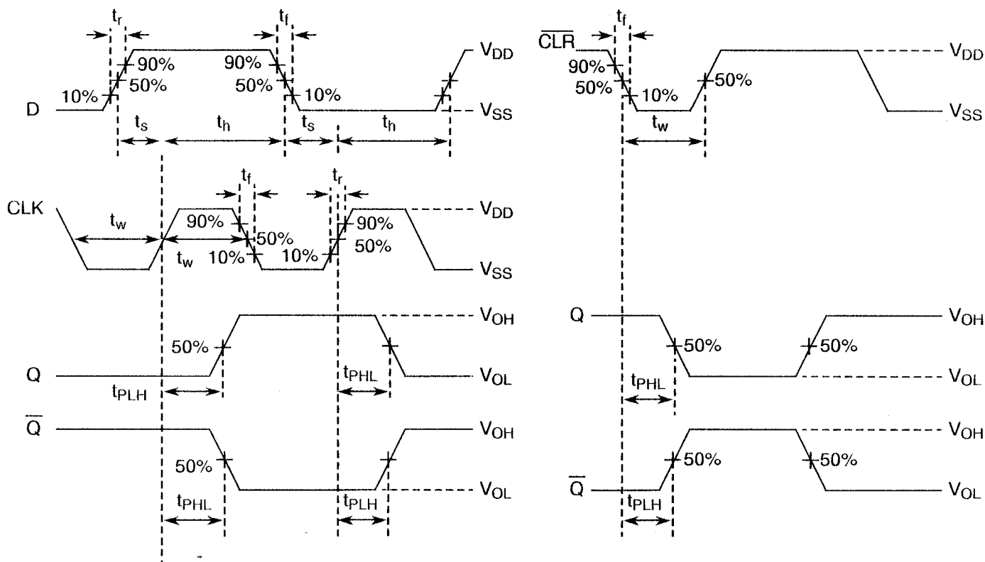
VOLTAGE WAVEFORMS
