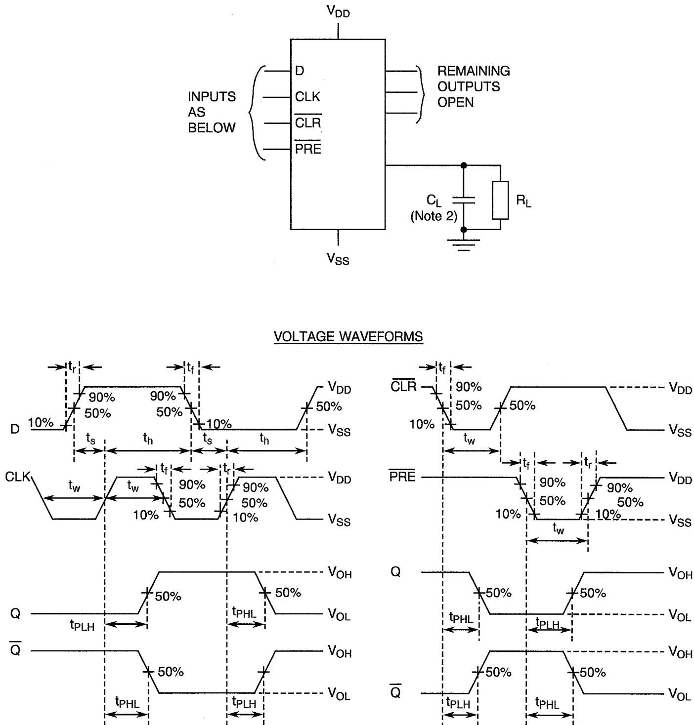
FIGURE 4(h) - PROPAGATION DELAY
