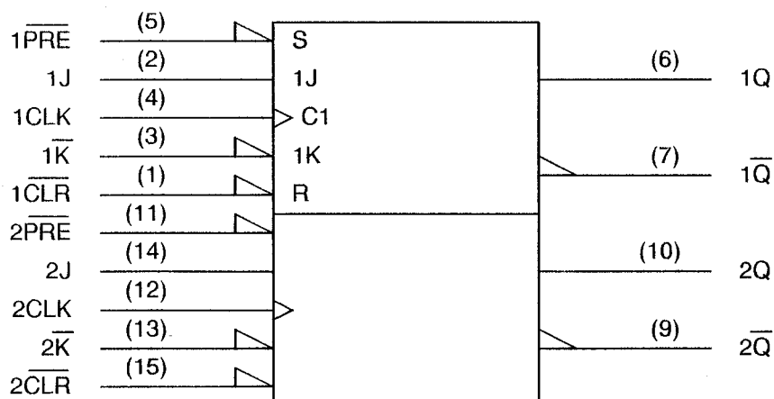
FIGURE 3(d) - FUNCTIONAL DIAGRAM
