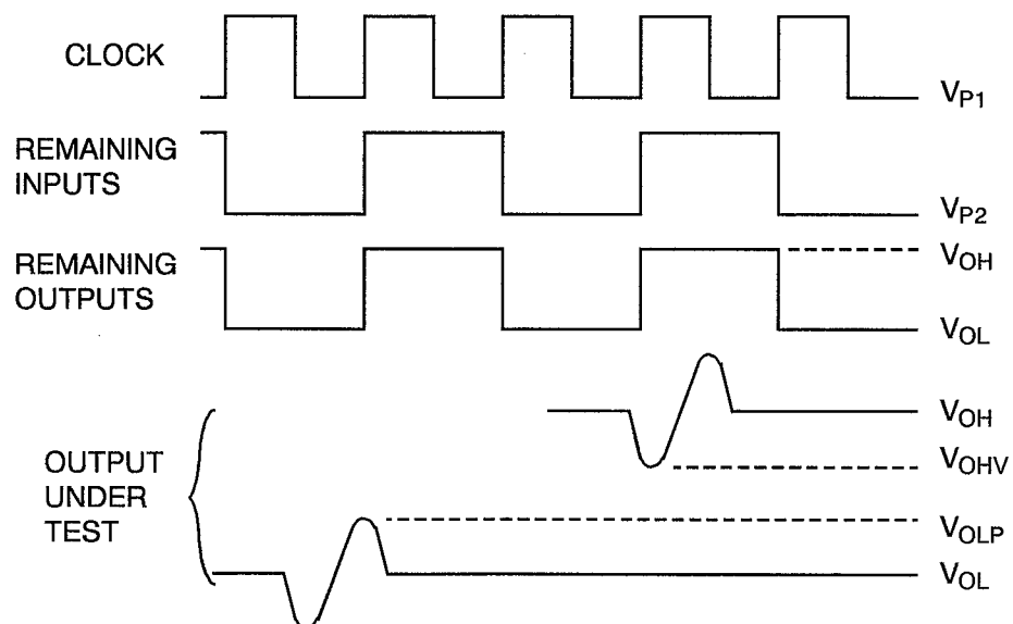
VOLTAGE WAVEFORMS
