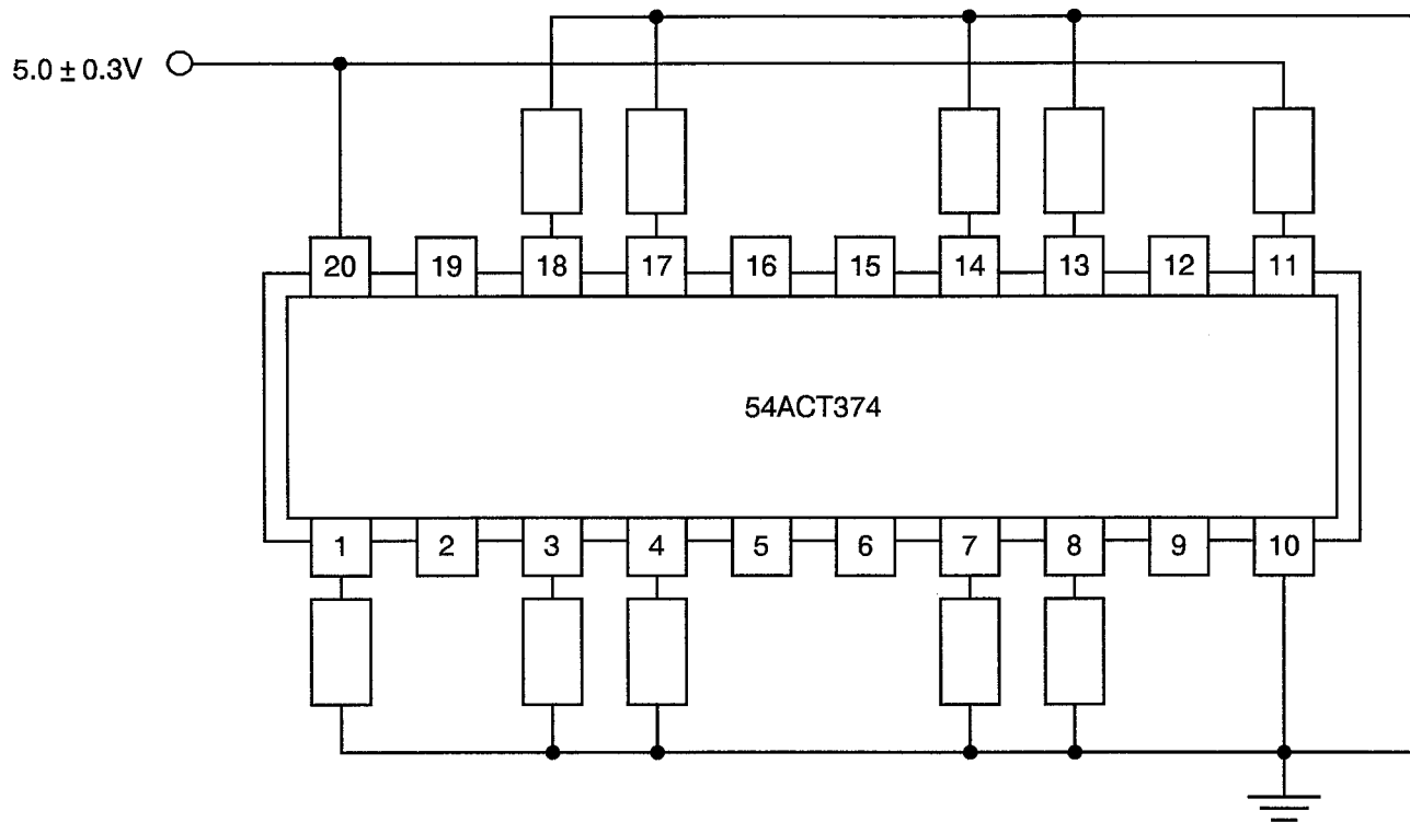
FIGURE 6 - BIAS CONDITIONS FOR IRRADIATION TESTING
