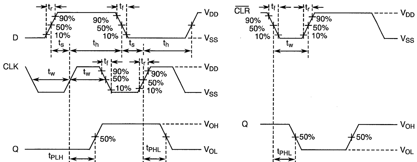
VOLTAGE WAVEFORMS
