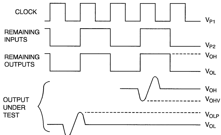
VOLTAGE WAVEFORMS
