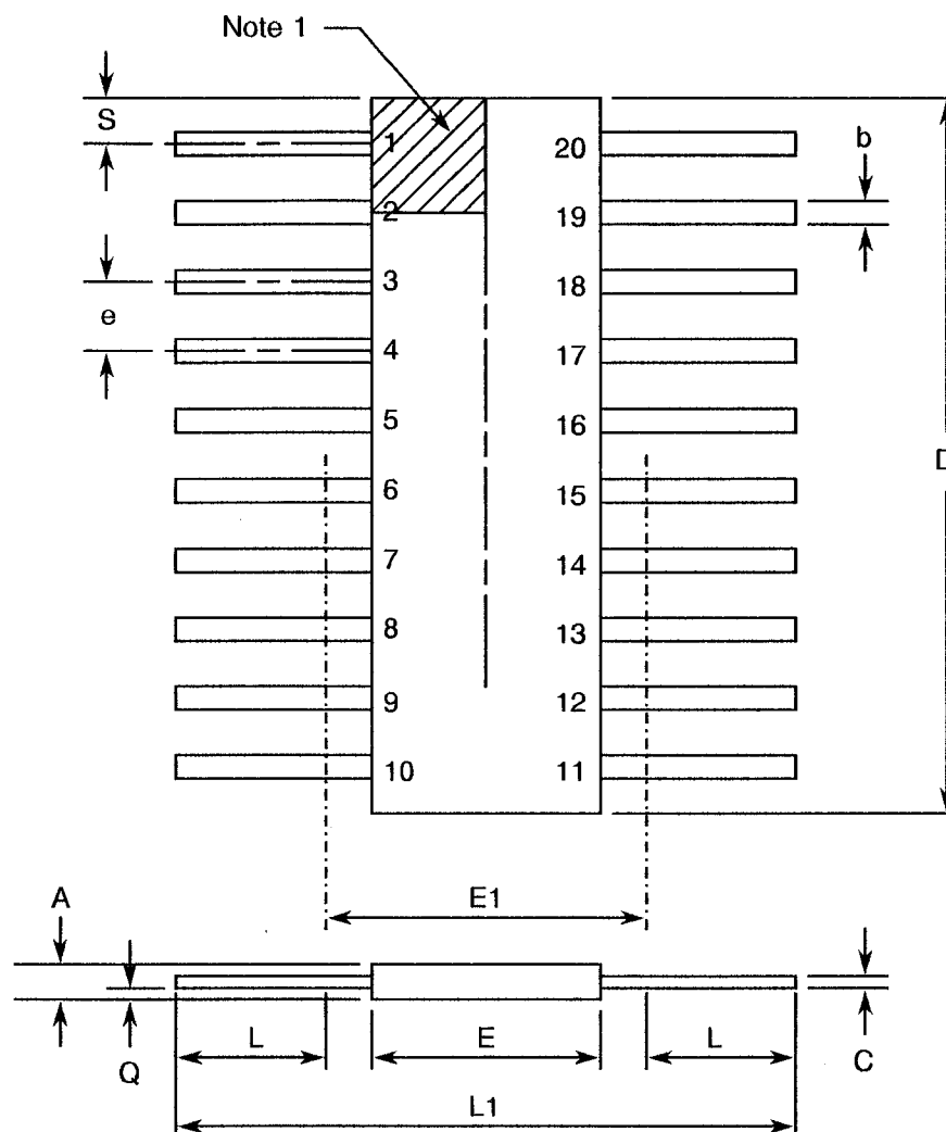
FIGURE 2(b) - FLAT PACKAGE, 20-PIN
