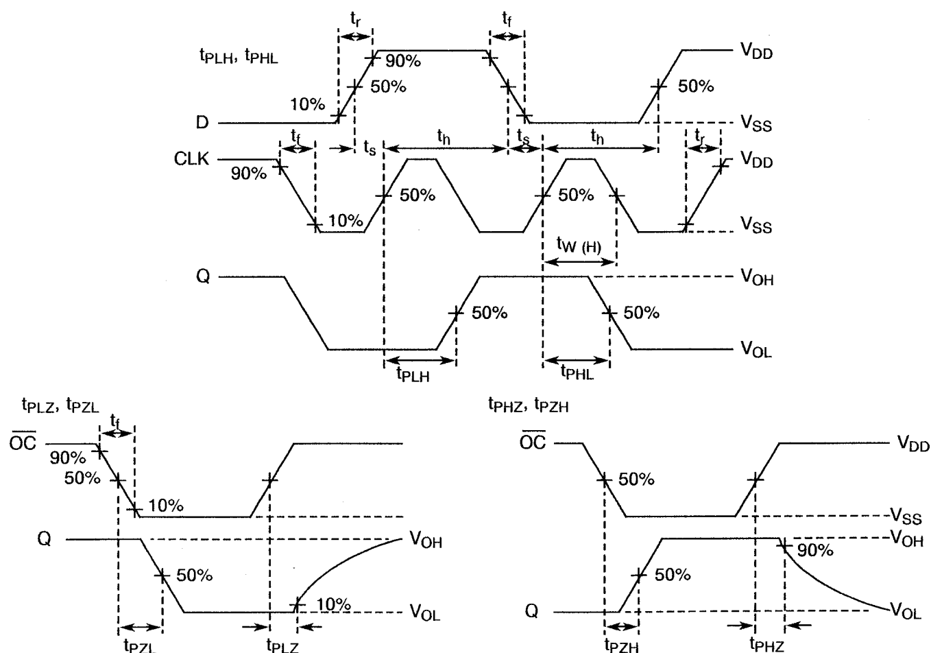
VOLTAGE WAVEFORMS
