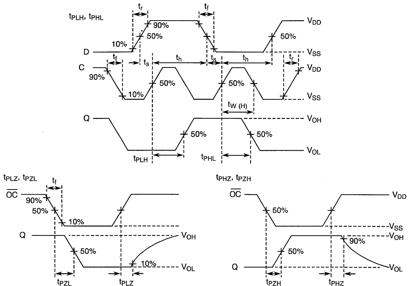
VOLTAGE WAVEFORMS
