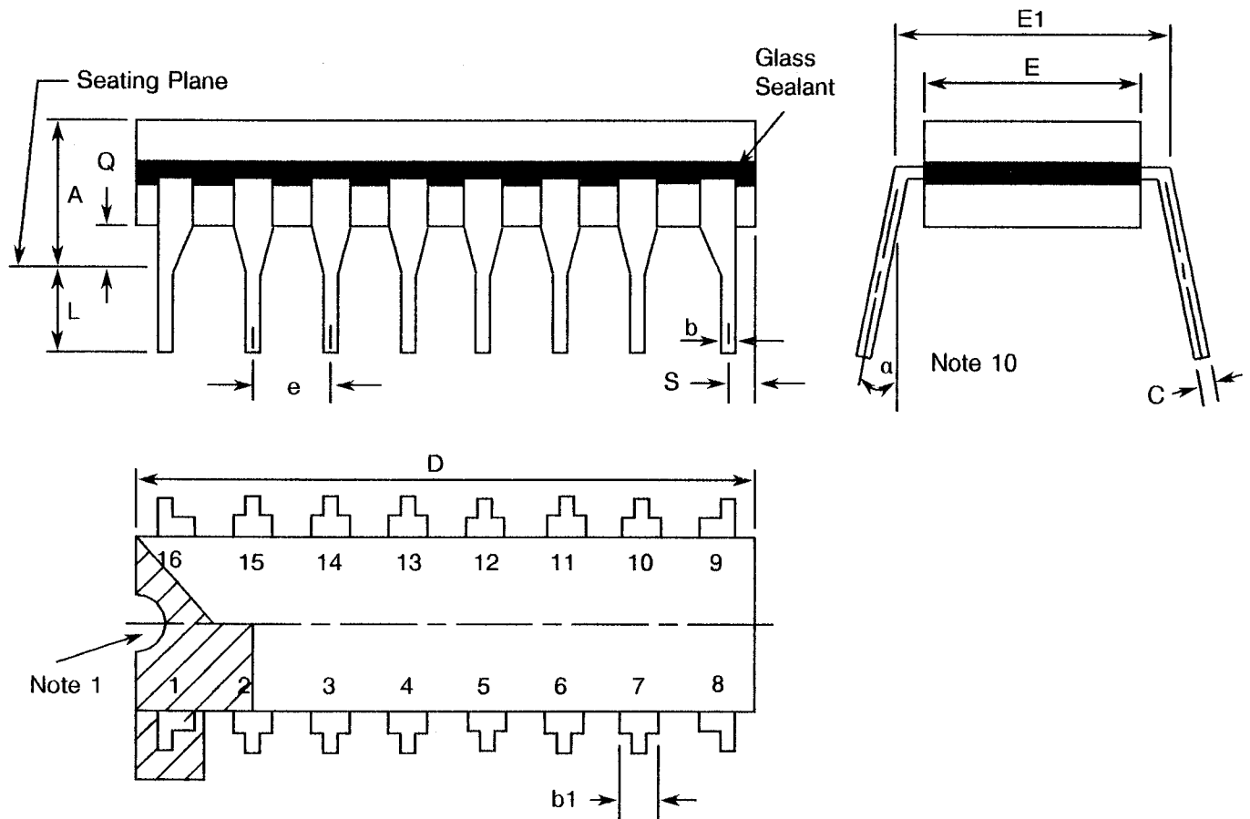
FIGURE 2(a) - DUAL-IN-LINE PACKAGE, 16-PIN
