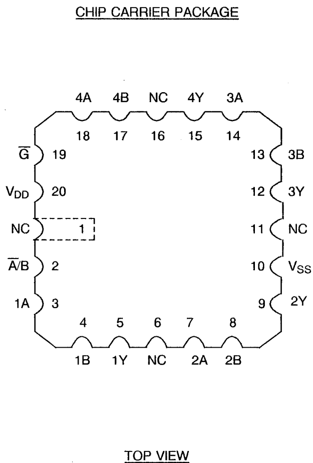
FIGURE 3(a) - PIN ASSIGNMENT
