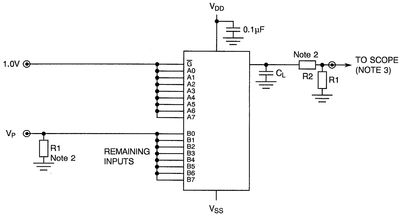
FIGURE 4(i) - GROUND BOUNCE
