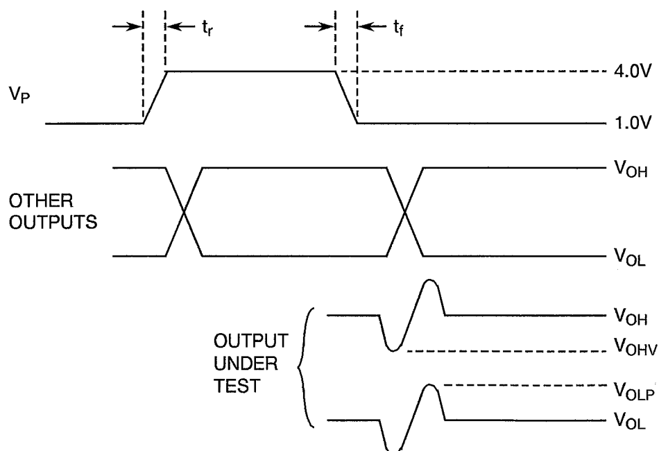
VOLTAGE WAVEFORMS
