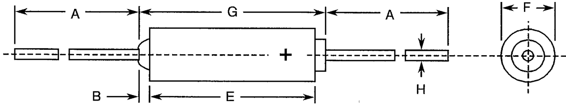
FIGURE 2 - PHYSICAL DIMENSIONS
