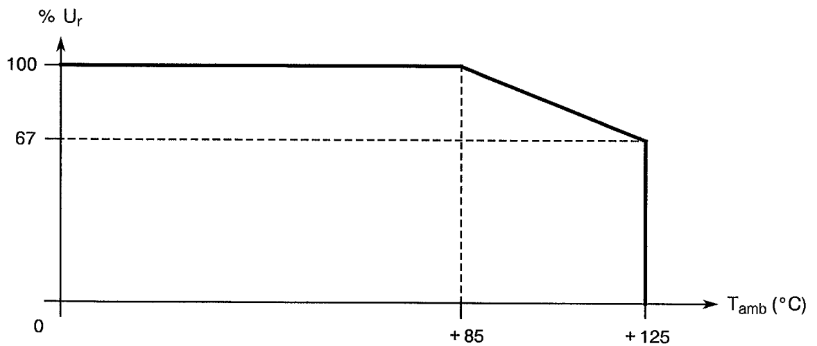
FIGURE 1 - PARAMETER DERATING INFORMATION
