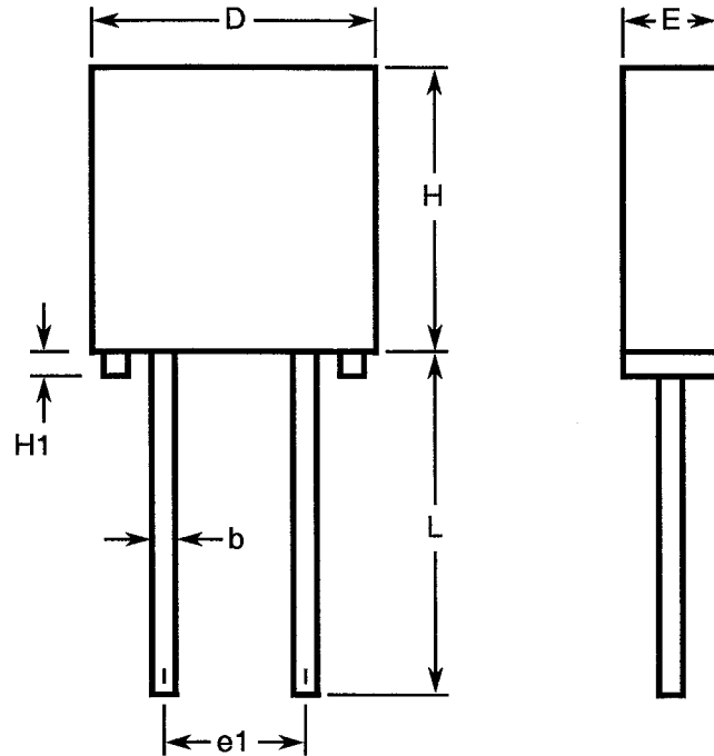
FIGURE 2 - PHYSICAL DIMENSIONS
