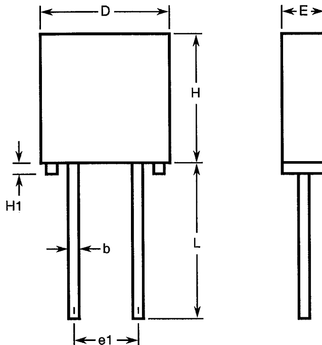
FIGURE 2 - PHYSICAL DIMENSIONS
