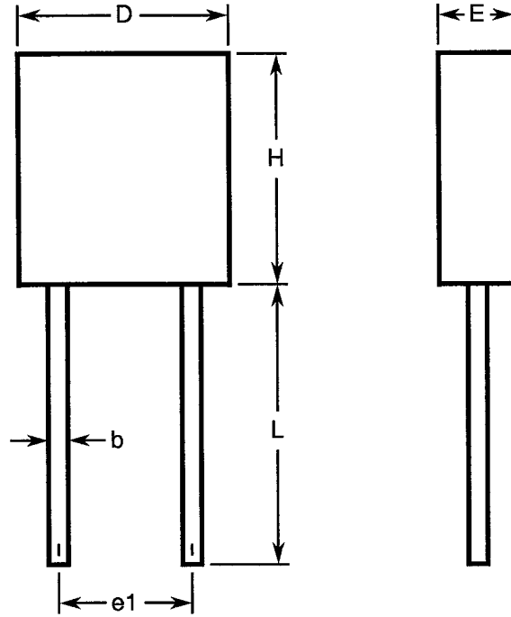
FIGURE 2 - PHYSICAL DIMENSIONS
