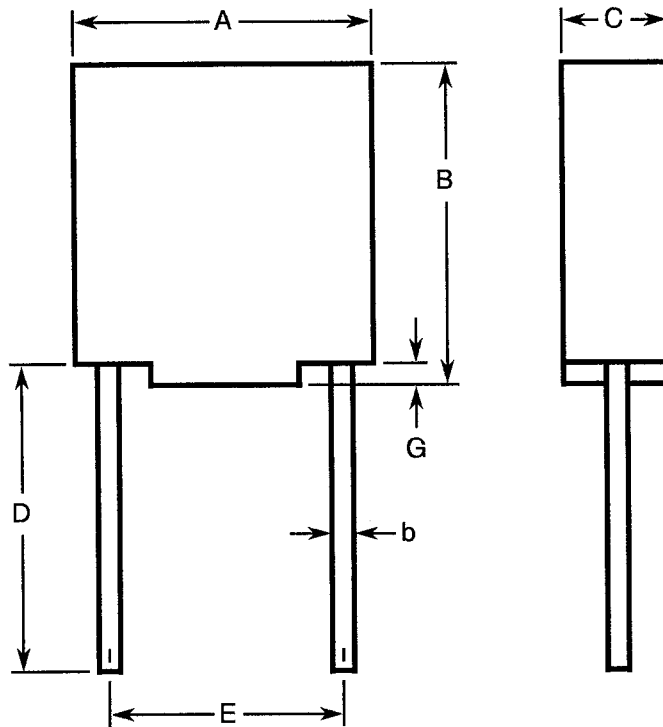
FIGURE 2 - PHYSICAL DIMENSIONS
