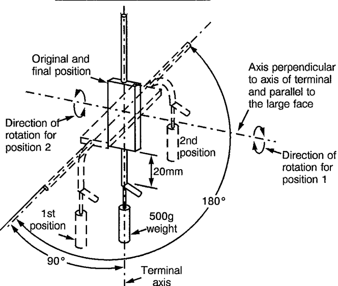
FIGURE I - BEND TEST
