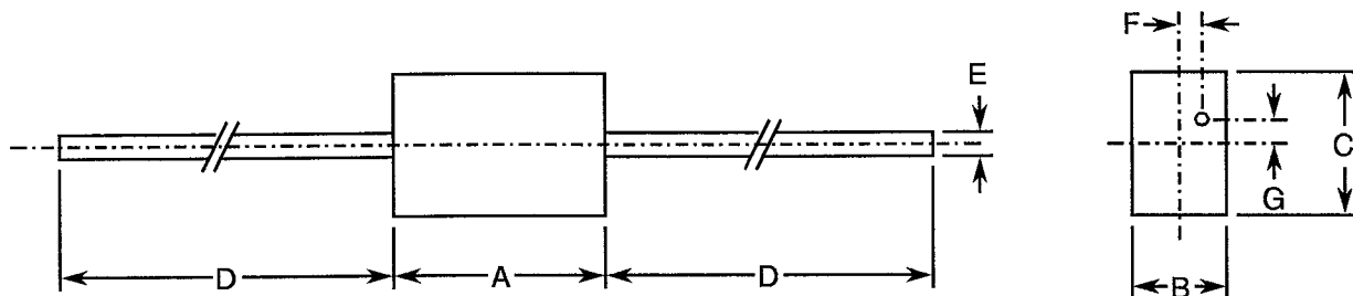
FIGURE 2 - PHYSICAL DIMENSIONS
