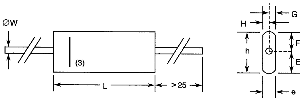
FIGURE 2 - PHYSICAL DIMENSIONS
