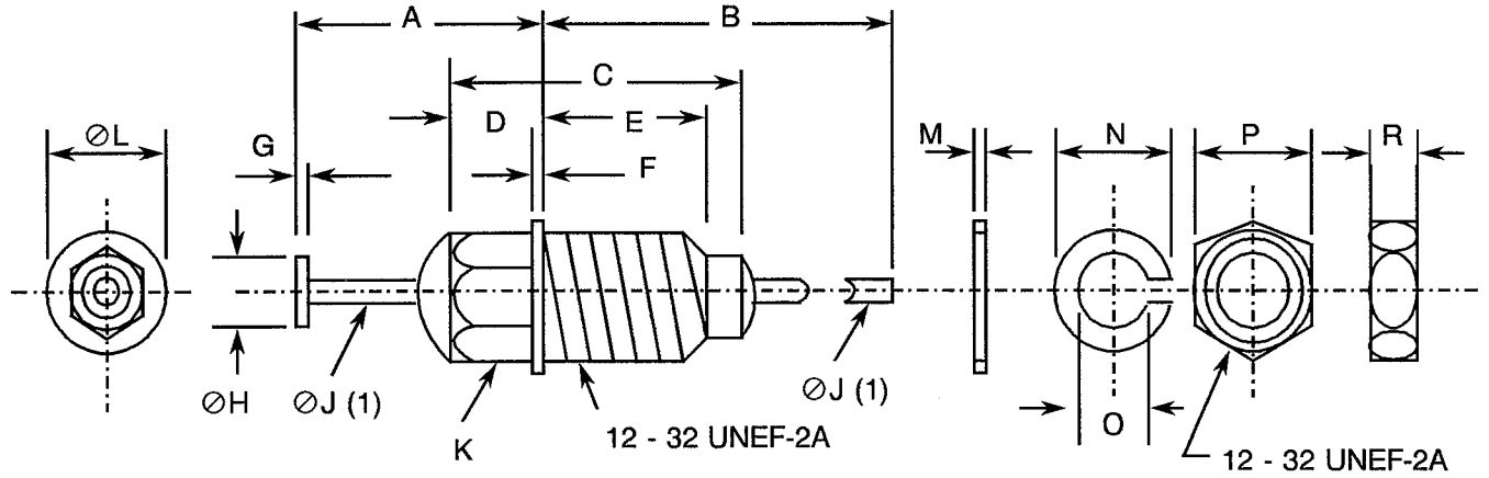
FIGURE 2 - PHYSICAL DIMENSIONS
