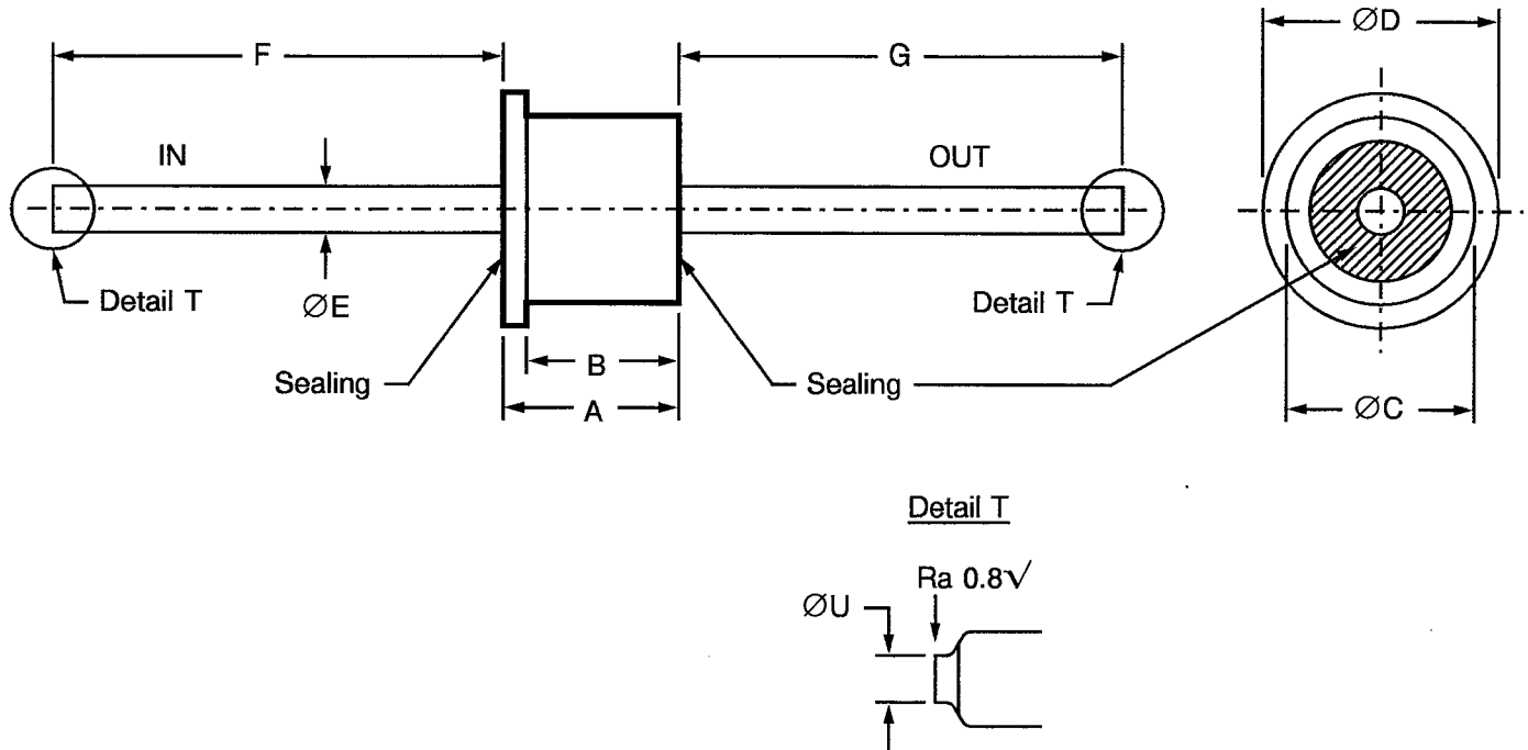
FIGURE 2 - PHYSICAL DIMENSIONS
