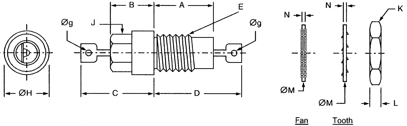
FIGURE 2 - PHYSICAL DIMENSIONS
