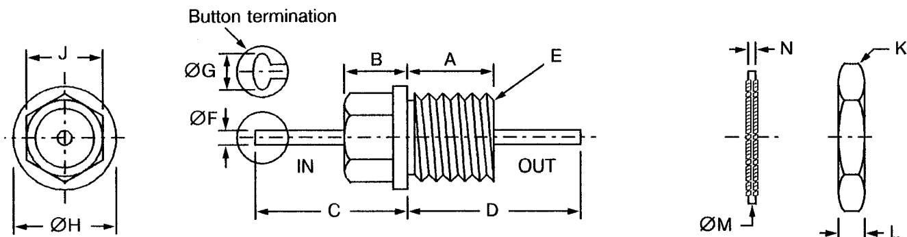
FIGURE 2 - PHYSICAL DIMENSIONS
