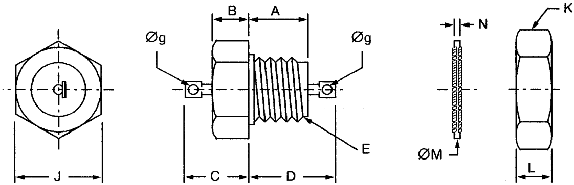
FIGURE 2 - PHYSICAL DIMENSIONS
