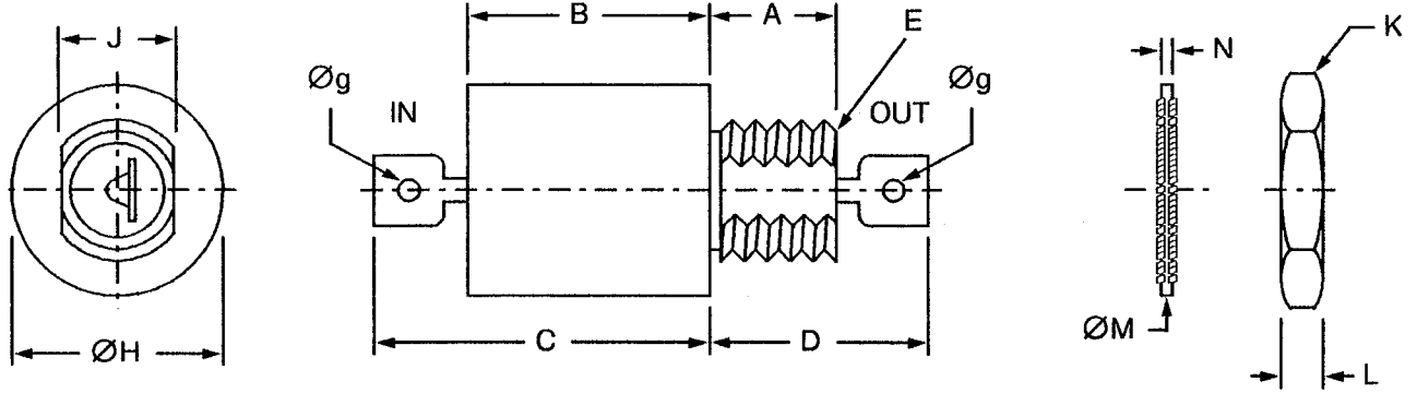
FIGURE 2 - PHYSICAL DIMENSIONS
