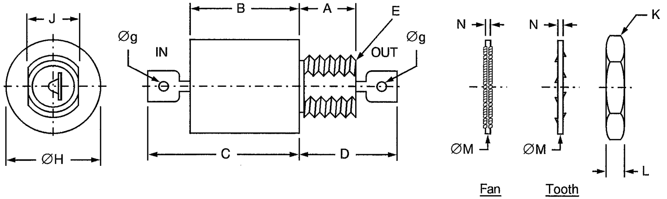
FIGURE 2 - PHYSICAL DIMENSIONS
