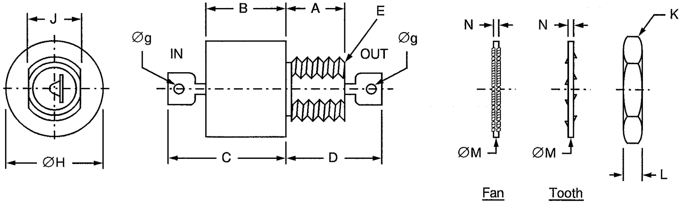
FIGURE 2 - PHYSICAL DIMENSIONS
