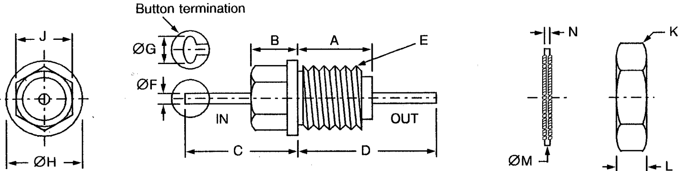
FIGURE 2 - PHYSICAL DIMENSIONS
