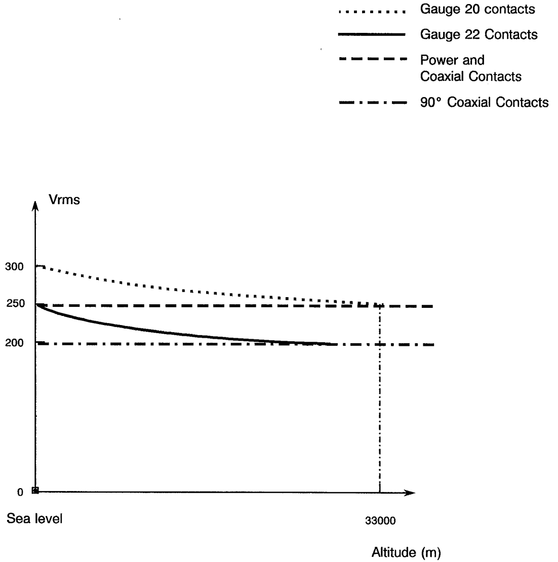
Working Voltage versus Altitude
