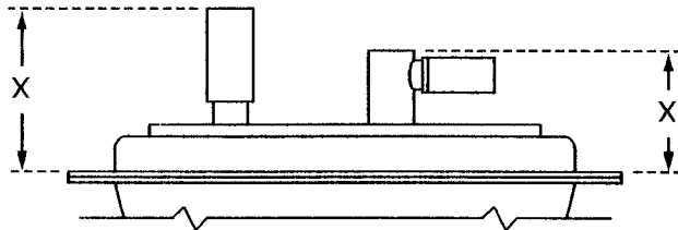
Maximum protrusion of contacts relative to rear of shell flange See Page 11 for value of X.
