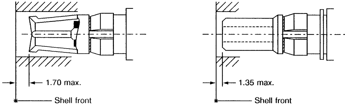
Maximum recess of contacts relative to front of shell
