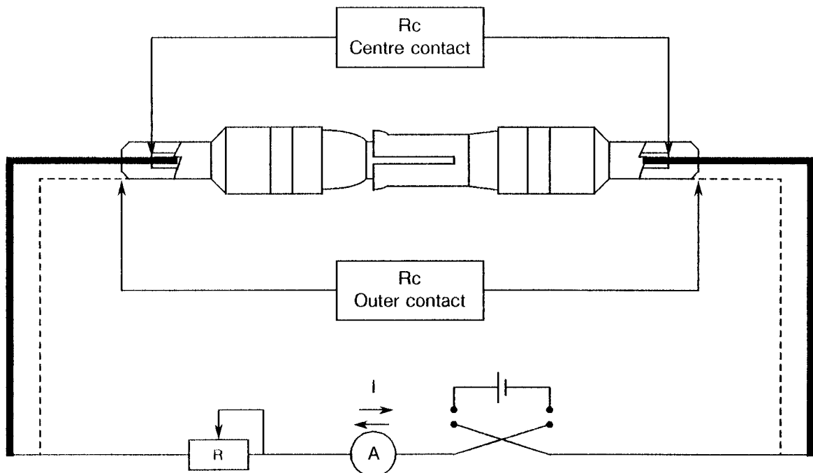
FIGURE 3 - TEST CIRCUIT FOR CONTACT RESISTANCE MEASUREMENT
