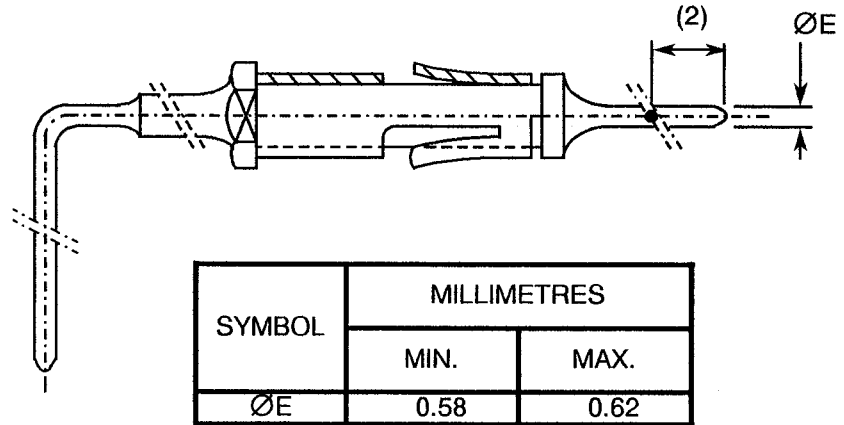
VARIANT 04 - CRIMP MALE CONTACT
