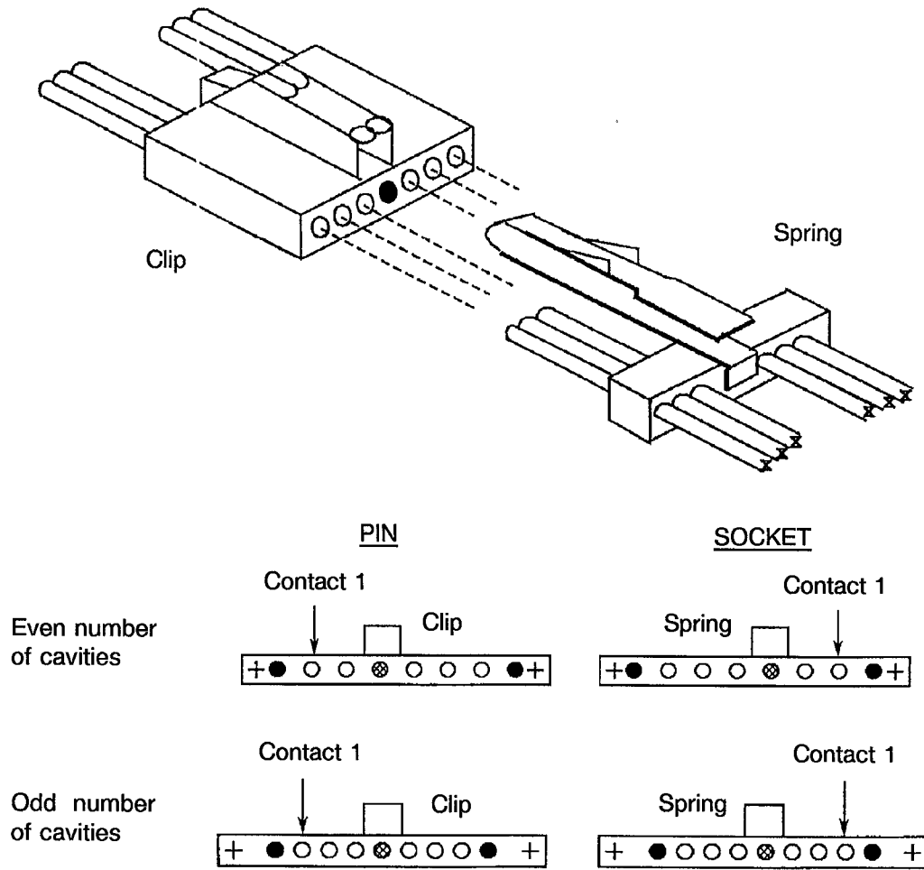
FIGURE 2.4 - LATCHING
