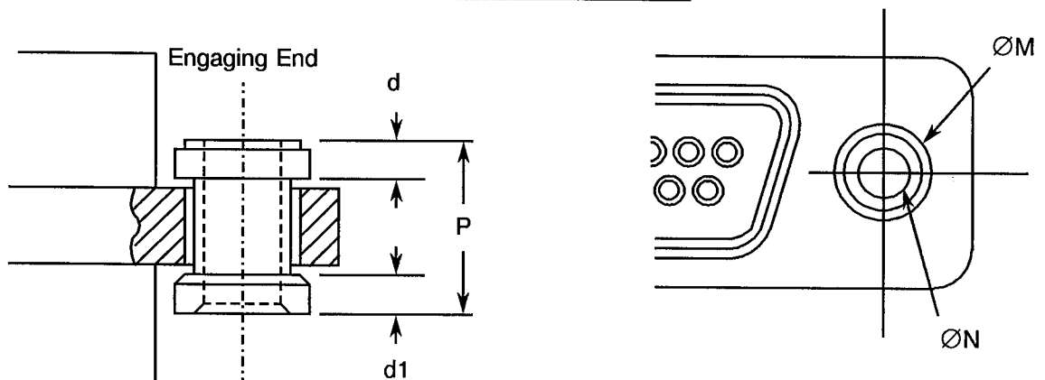
FIGURE 2-6 - FLOATING MOUNT
