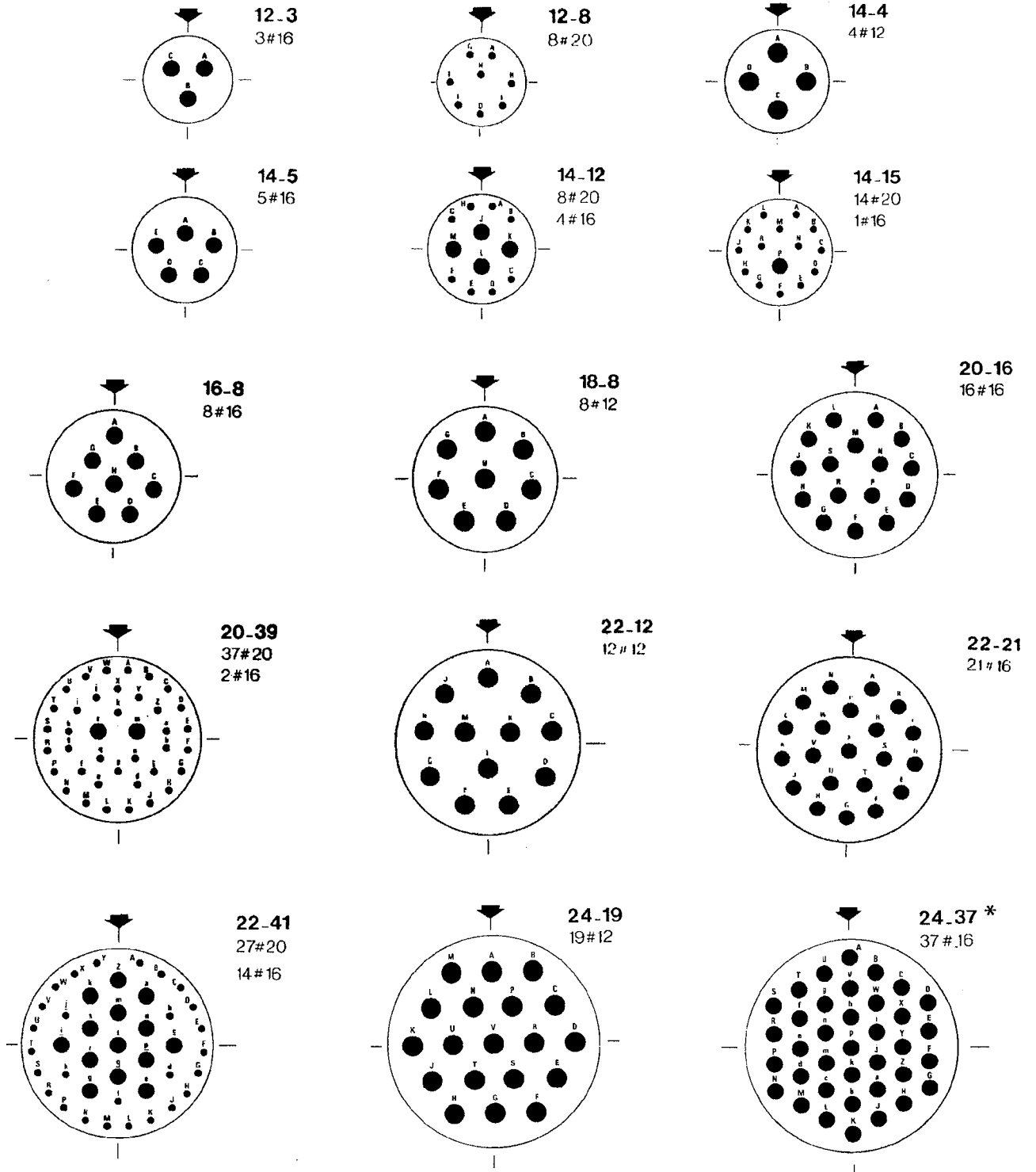
FIGURE 2(b) - PHYSICAL DIMENSIONS SPECIAL CONTACT ARRANGEMENTS - FRONT VIEW PIN INSERT
