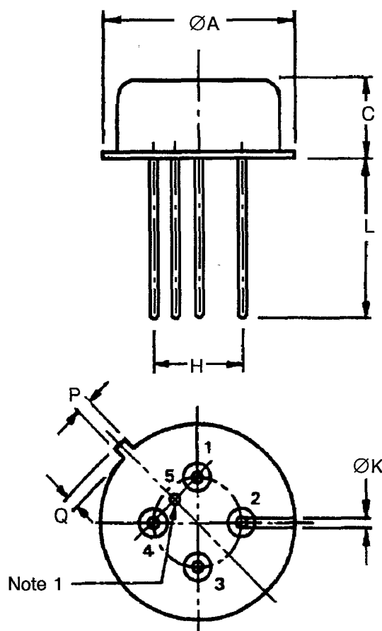
FIGURE 2 - PHYSICAL DIMENSIONS
