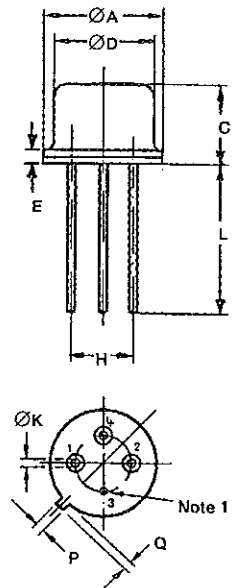
FIGURE 2(b) - 4-PIN PACKAGE
