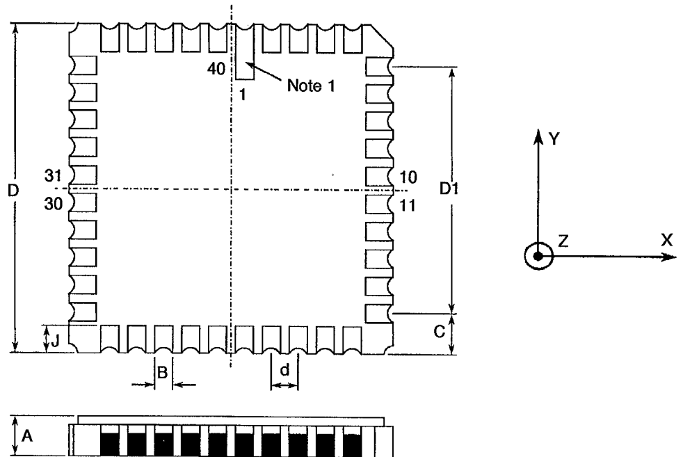
FIGURE 2 - PHYSICAL DIMENSIONS
