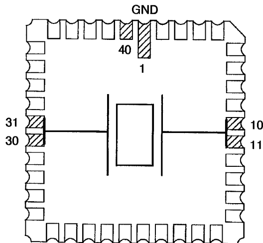
FIGURE 3 - FUNCTIONAL DIAGRAM
