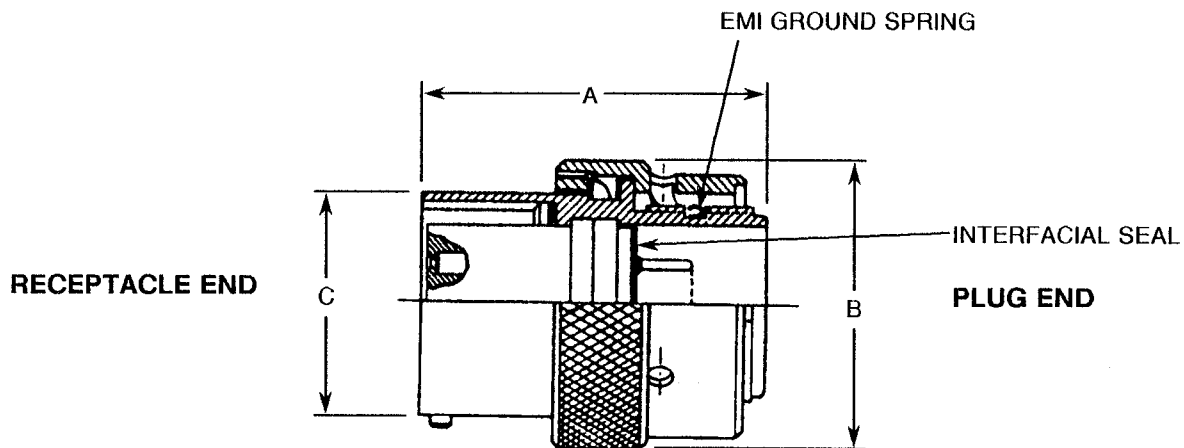
FIGURE 2(a) - SAVERS TYPE VARIANT 01 - SAVERS FOR 3401/052 CONNECTORS (SERIES I)
