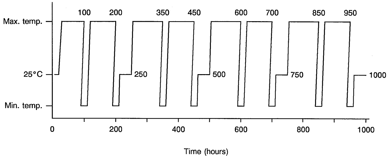
FIGURE II - AMBIENT TEMPERATURES
