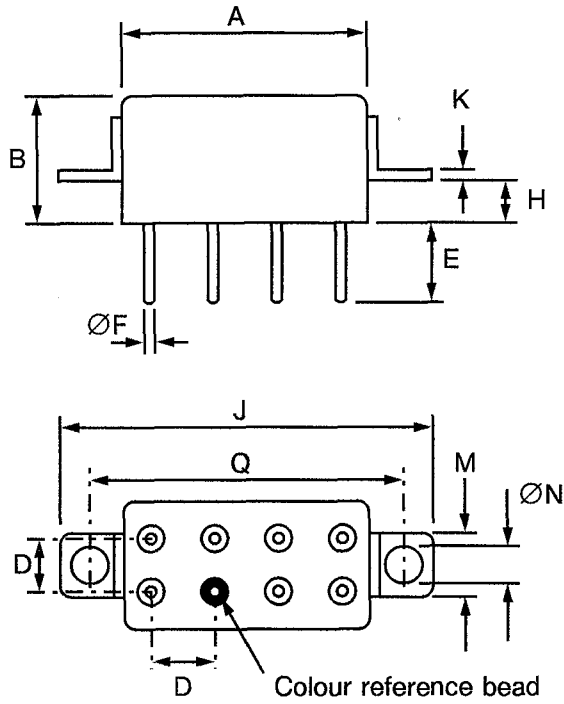
FIGURE 2(b) - VARIANT 02, RELAY WITH PLUG-IN TERMINALS AND HORIZONTAL SHOULDER BRACKETS
