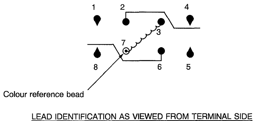
FIGURE 3 - CIRCUIT SCHEMATIC
