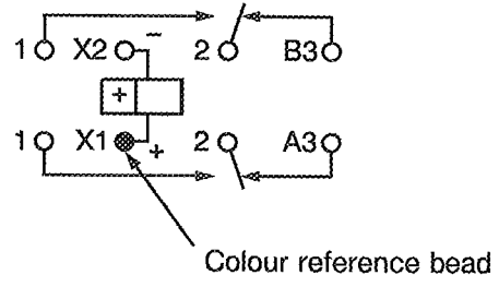
FIGURE 3 - CIRCUIT SCHEMATIC
