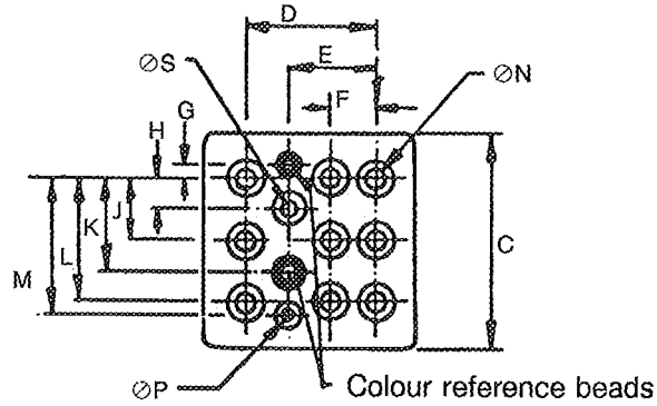
FIGURE 2(d) - VARIANTS 05 AND 15, RELAY WITH STRAIGHT TERMINALS AND PLAIN CASE
