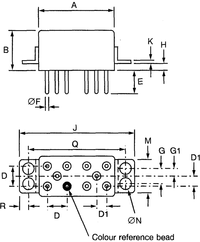
FIGURE 2(g) - VARIANT 07, RELAY WITH PLUG-IN TERMINALS AND HORIZONTAL SHOULDER BRACKETS (4 HOLES)
