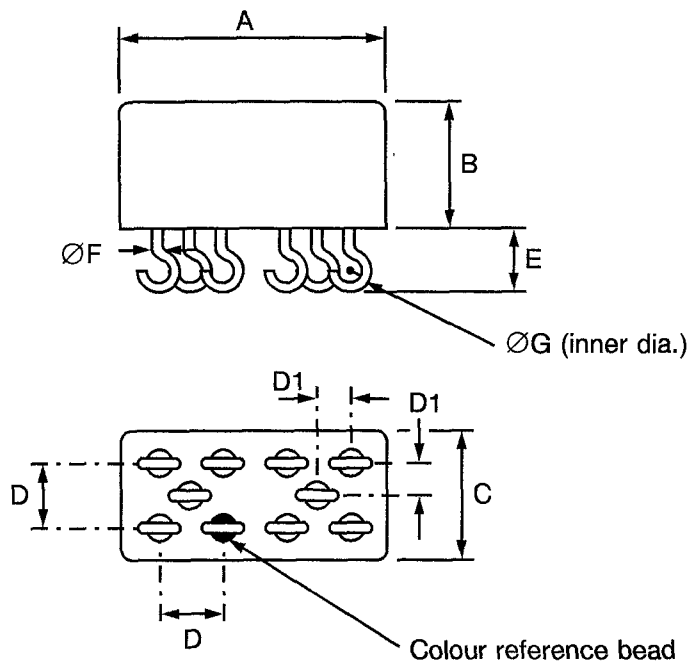
FIGURE 2(e) - VARIANT 05, RELAY WITH SOLDERABLE, HOOK-END TERMINALS AND PLAIN CASE
