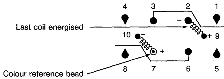
FIGURE 3 - CIRCUIT SCHEMATIC
