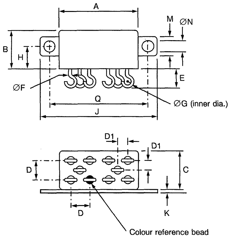
FIGURE 2(c) - VARIANT 03, RELAY WITH SOLDERABLE, HOOK-END TERMINALS AND VERTICAL SHOULDER BRACKETS
