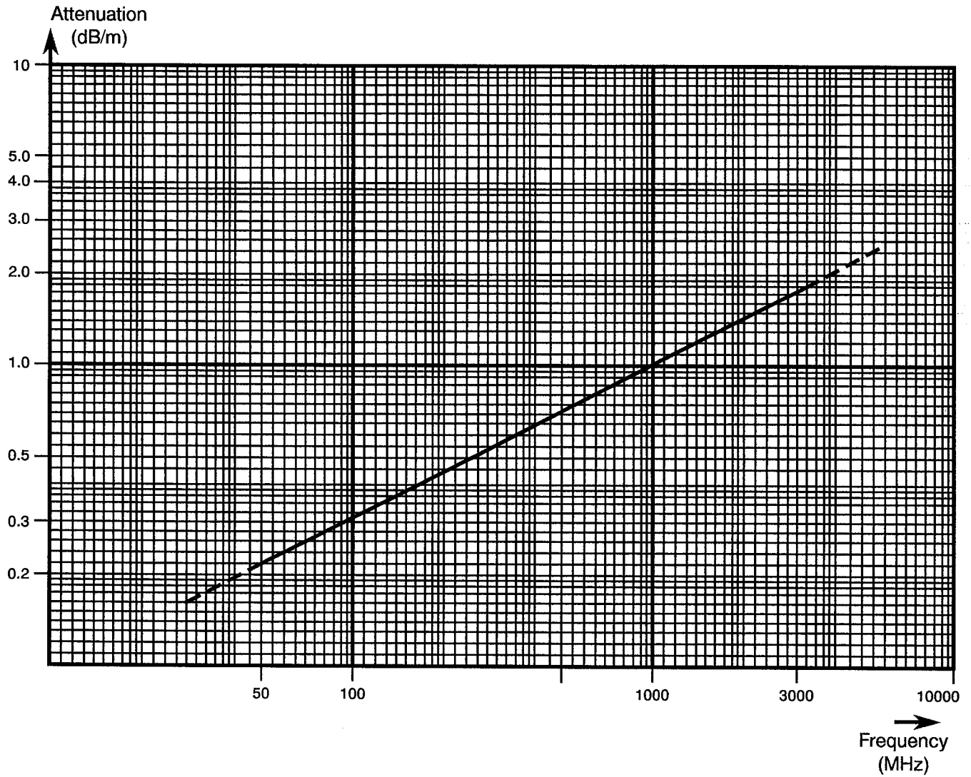
FIGURE 1(b) - MAXIMUM ATTENUATION
