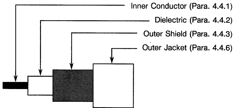
FIGURE 2(b) - DOUBLE SHIELD COAXIAL CABLE VARIANT 02
