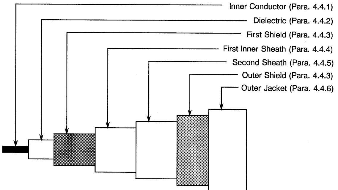
FIGURE 2(c) - SHIELDED AND JACKETED COAXIAL CABLE VARIANT 03
