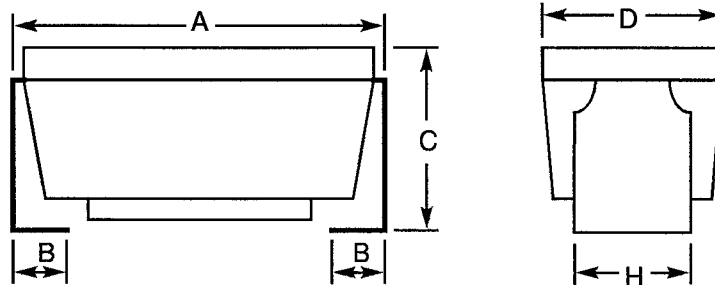
FIGURE 2 - PHYSICAL DIMENSIONS
